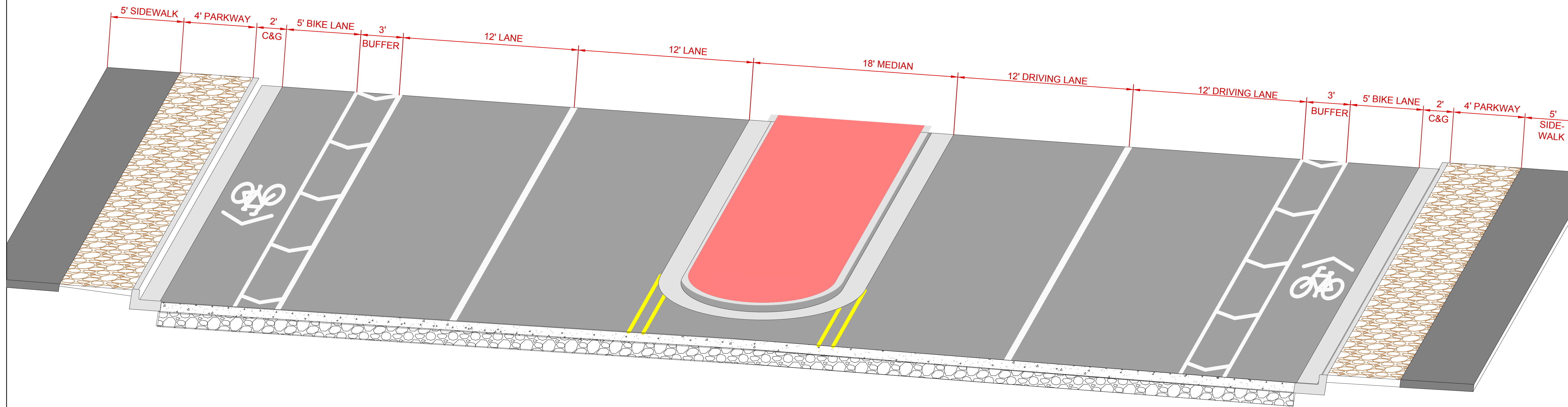
VALLEY DRIVE & AVE. DE MESILLA CORRIDOR STUDY TYPICAL SECTION G
